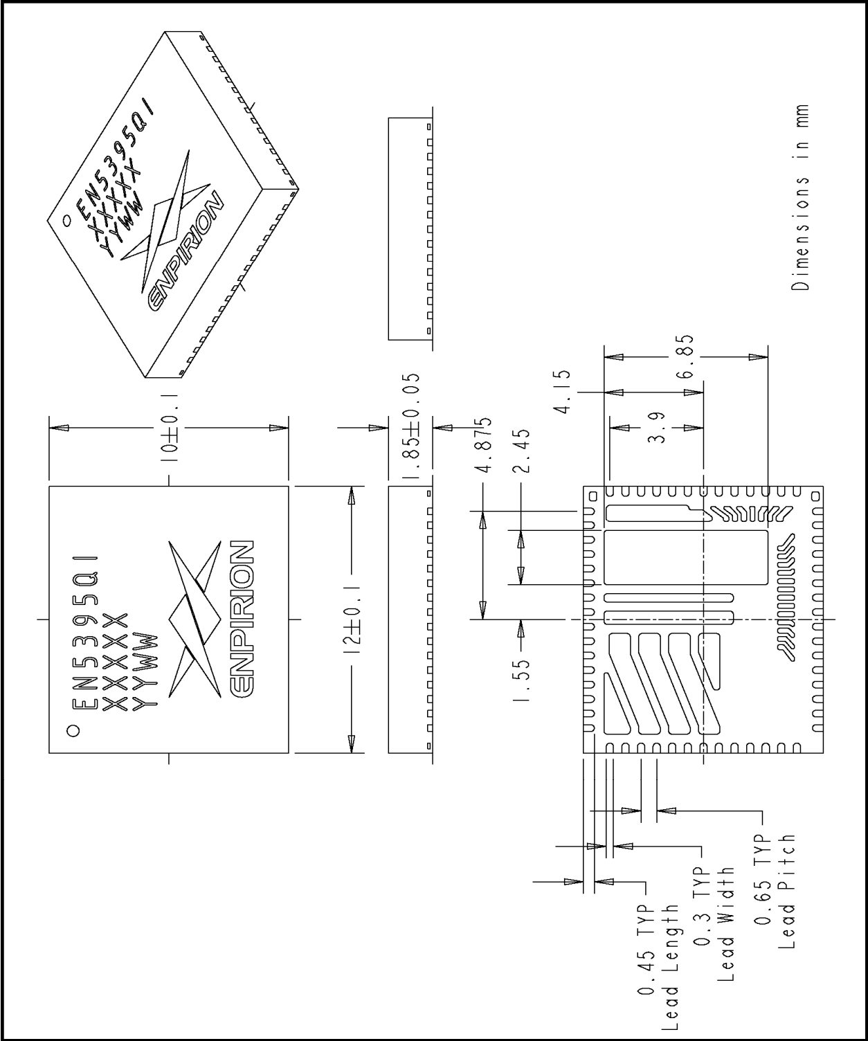
Figure 1: EN5395QI Package Outline Drawing
