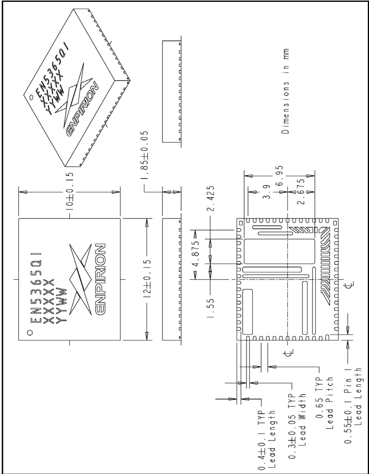
Figure 1: EN5365QI Package Outline Drawing
