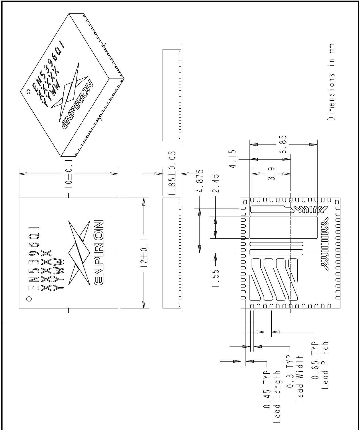
Figure 1: EN5396QI Package Outline Drawing
